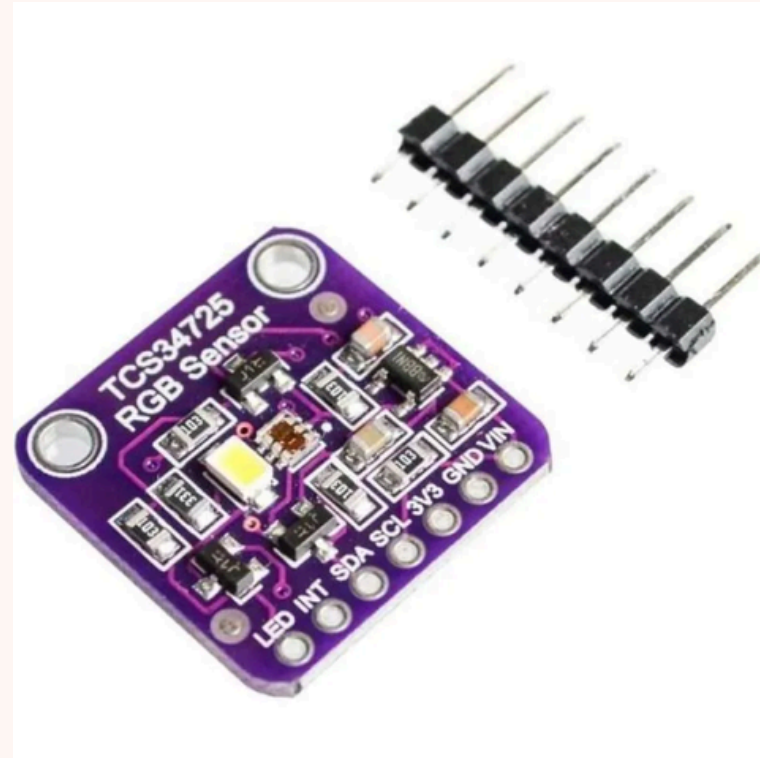
Sensor RGB TCS34725
