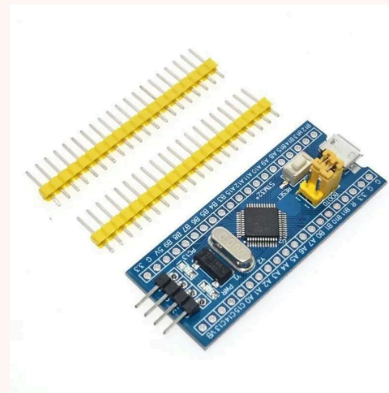
STM 32 SDA: PB7 | SCL: PB6
